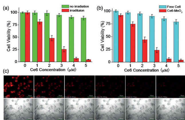
Figure 2. a) Cytotoxicity of Ce6-MnO 2 nanosystem with Ce6 at different concentrations in the presence or absence of irradiation. b) Phototoxicity of free Ce6 and Ce6-MnO 2 nanosystem with Ce6 at different concentrations. c) Real-time fluorescence images and morphology of MCF-7 cells treated with Ce6-MnO 2 nanosystem and laser at 405 nm (top) and bright-field images (bottom). Concentration of MnO 2 nanosheets in these studies was 41.76 μg mL -1 .
