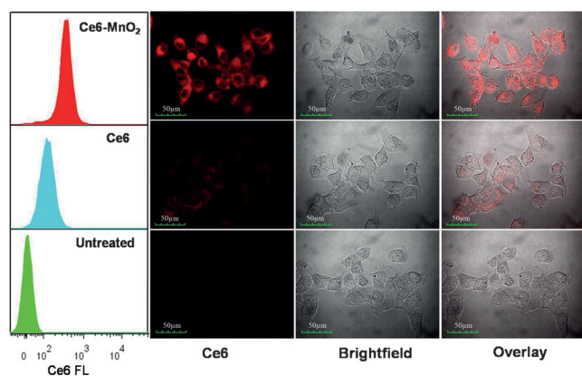
Figure 1. Flow cytometry analysis (left) and confocal fluorescence images (right) of MCF-7 cells treated with free Ce6 and Ce6-MnO 2 nanosystem. Concentrations of Ce6 and MnO 2 nanosheets were 1 μM and 41.76 μg mL -1 , respectively.
