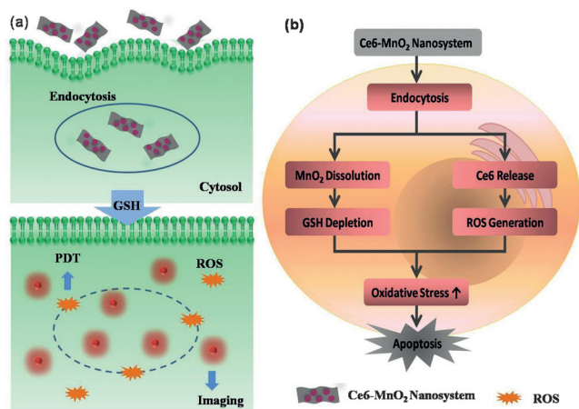
Scheme 1. Activation mechanism of the Ce6-MnO 2 nanosystem for highly efficient photodynamic therapy. The nanosheet can adsorb and efficiently deliver photosensitizers into cells and protect them from self-destruction upon light irradiation. Once endocytosed, the nanosystem is disintegrated upon reduction of MnO 2 nanosheets by intracellular GSH, simultaneously releasing Ce6 for fluorescence imaging and decreasing the level of GSH for highly efficient PDT.
