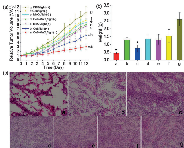
Figure 4. a) Tumor growth curves of different groups of tumor-bearing mice after treatment. Tumor volumes were normalized to their initial sizes. Error bars represent the standard deviations of 3 mice per group. Asterisk indicates P < 0.05 . Weight of tumors (b) and H&E stained tumor sections (c) collected from different groups of mice 12 days post-treatment.
