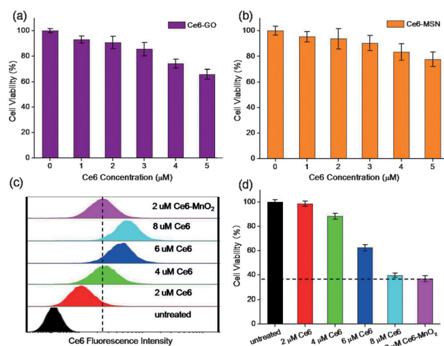
Figure 3. Phototoxicity of Ce6-GO (a) and Ce6-MSN (b) nanosystem on MCF-7 cells with Ce6 at different concentrations as indicated. c) Flow cytometry analysis of MCF-7 cells treated with Ce6-MnO 2 nanosystem and different concentrations of free Ce6. d) Cytotoxicity of MCF-7 cells treated with Ce6-MnO 2 nanosystem and different concentrations of free Ce6. Concentration of MnO 2 nanosheets in these studies was 41.76 μg mL -1 .
